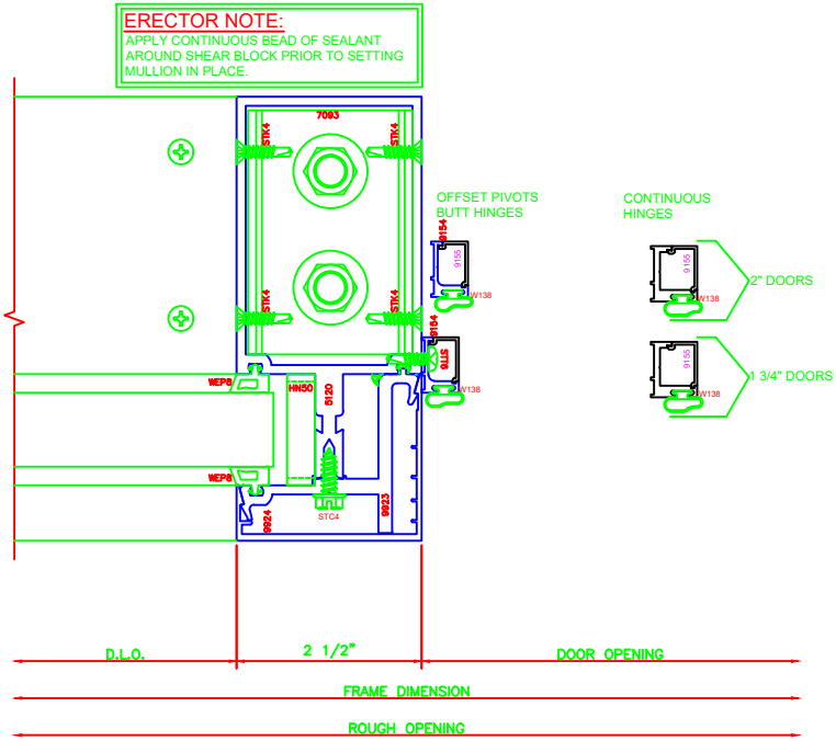
825 O.G. VERT. 5600 6"
